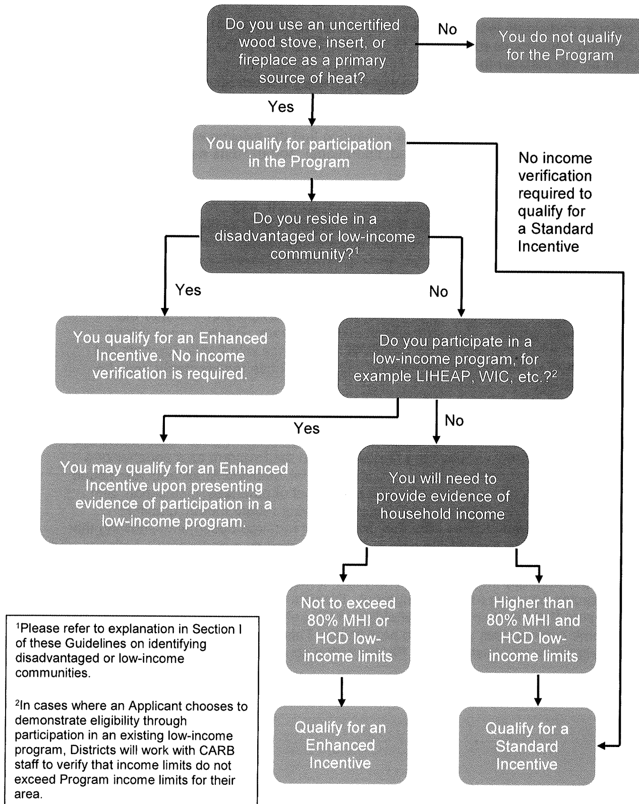
Figure 2. Approval Process
